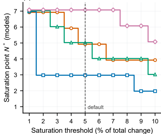
(a) Raw CMIP6
